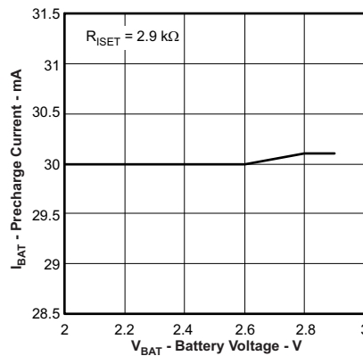
Figure 17. PRECHARGE CURRENT vs BATTERY VOLTAGE
